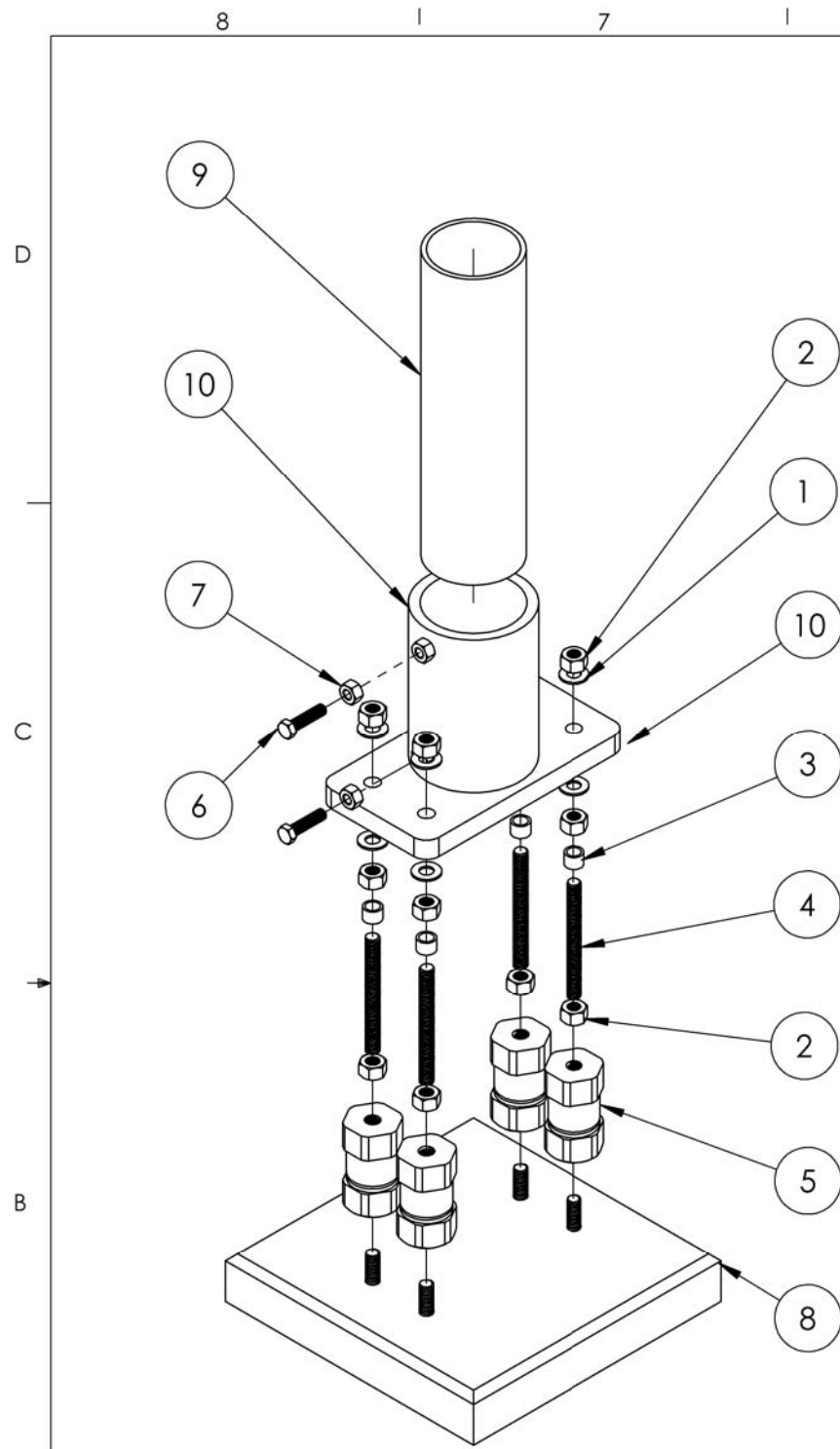
EXPLODED VIEW
